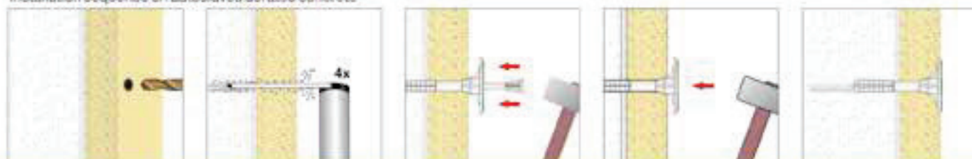
Installation sequence on autoclaved aerated concrete
